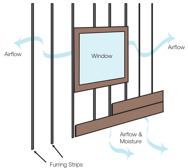
SINGLE HORIZONTAL ROW OF QUARRIX FURRING
